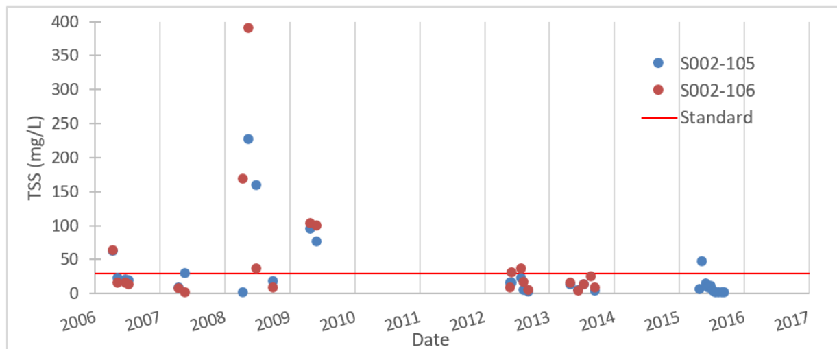
Figure 2. TSS data for Hay Creek from 2006 through 2015 (TMDL information)
